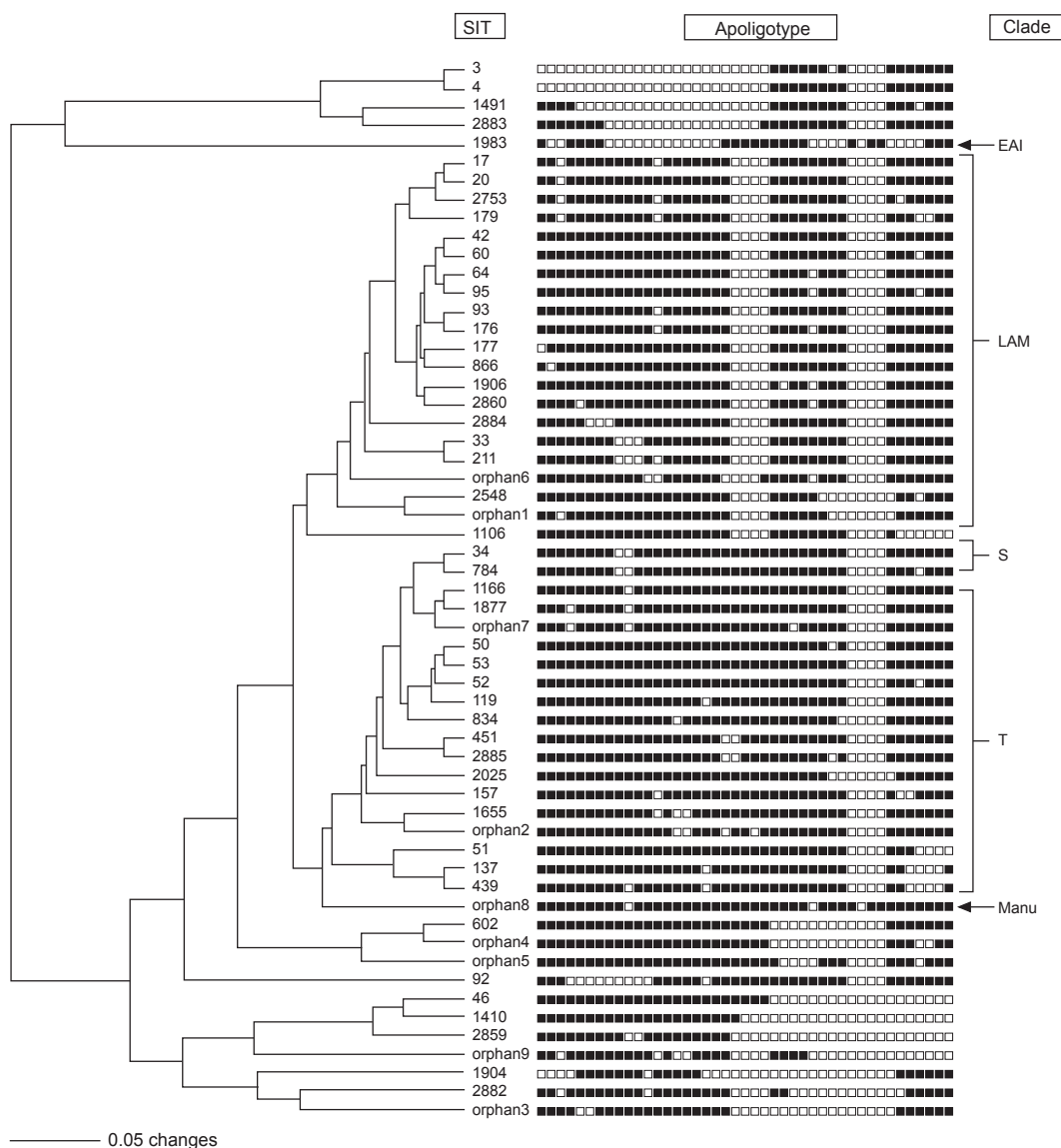
Tree of spoligotype patterns Mycobacterium tuberculosis isolates (n = 57 profiles) by using the Phylogenetic Analysis Using Parsimony 4.0b software and the unweighted pair group method with arithmetic mean method. EAI: East-African-Indian; LAM: Latin-American-Mediterranean; SIT: Spoligotype International Type as defined in the international database of the Institute Pasteur de la Guadeloupe.
