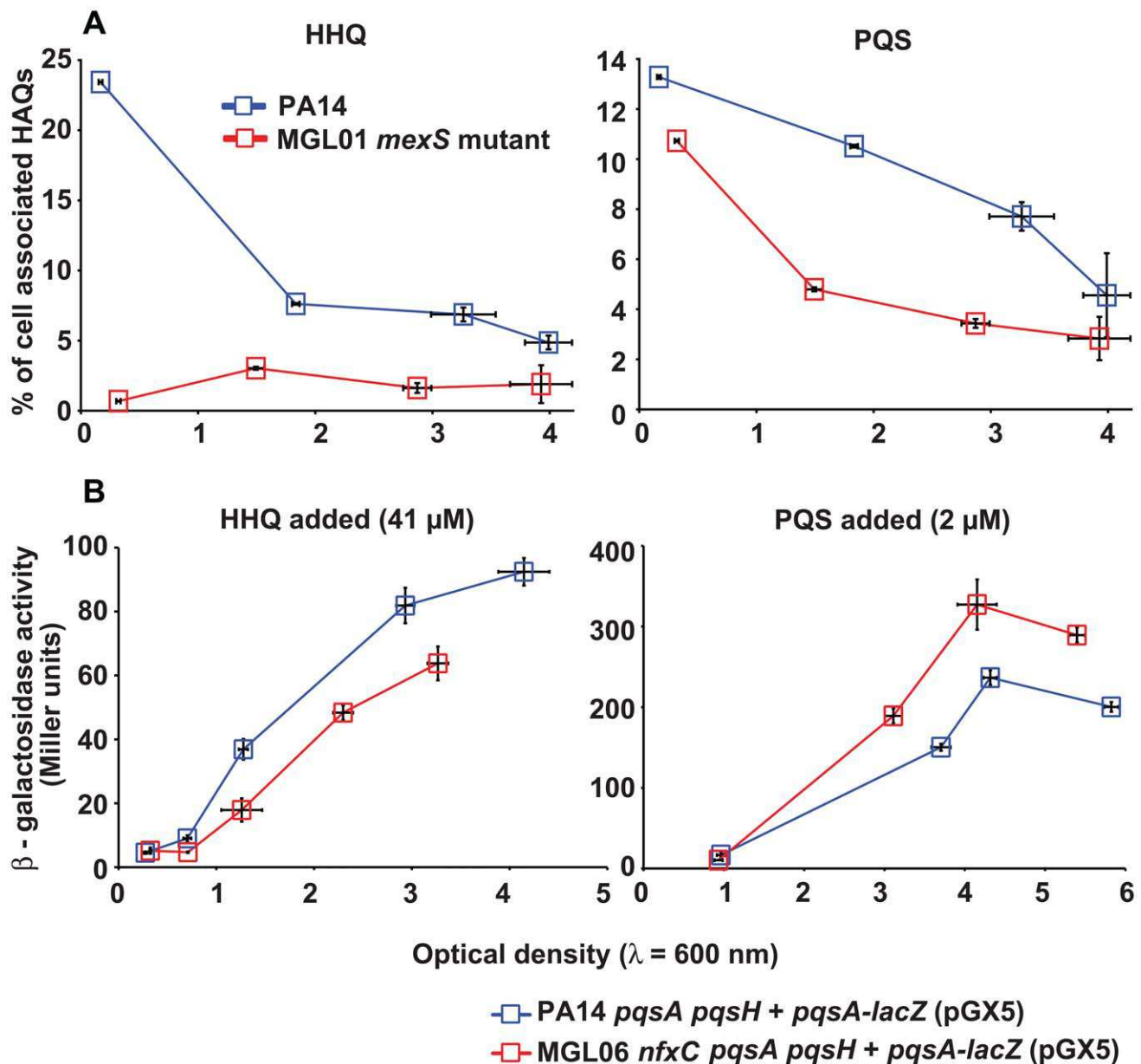
Figure 4. HHQ is exported out of constitutively expressing MexEF-OprN efflux cells (MGL01). (A) Shown is the percentage of cell-associated HHQ or PQS as a function of cell growth ( OD_{600} ). Here, we show that MGL01 cells contain less cell-associated HHQ and PQS when compared to the PA14 wild-type strain. This is in contrast with the observation that HHQ concentrations are higher in MGL01 than in PA14 cultures (Fig. 1). HAQs were quantified by LC-MS/MS and experiment was achieved using biological triplicates. (B) Shown is the \beta -galactosidase activity (Miller units) of a pqsA-lacZ transcriptional reporter as a function of cell growth ( OD_{600} ). This experiment was conducted in the presence of exogenously added HHQ (41 \mu M) or PQS (2 \mu M). Experiment was achieved using biological triplicates. doi:10.1371/journal.pone.0024310.g004
