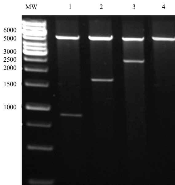
Fig. 6. Digestion of genes cloned in pET28a vector by NcoI-HindIII . MW: Molecular weight marker; Lane 1: Digested pET-fimH; Lane 2: Digested pET-fliC; Lane 3: Digested pET-fimH/fliC; Lane 4: pET28a Undigested.
