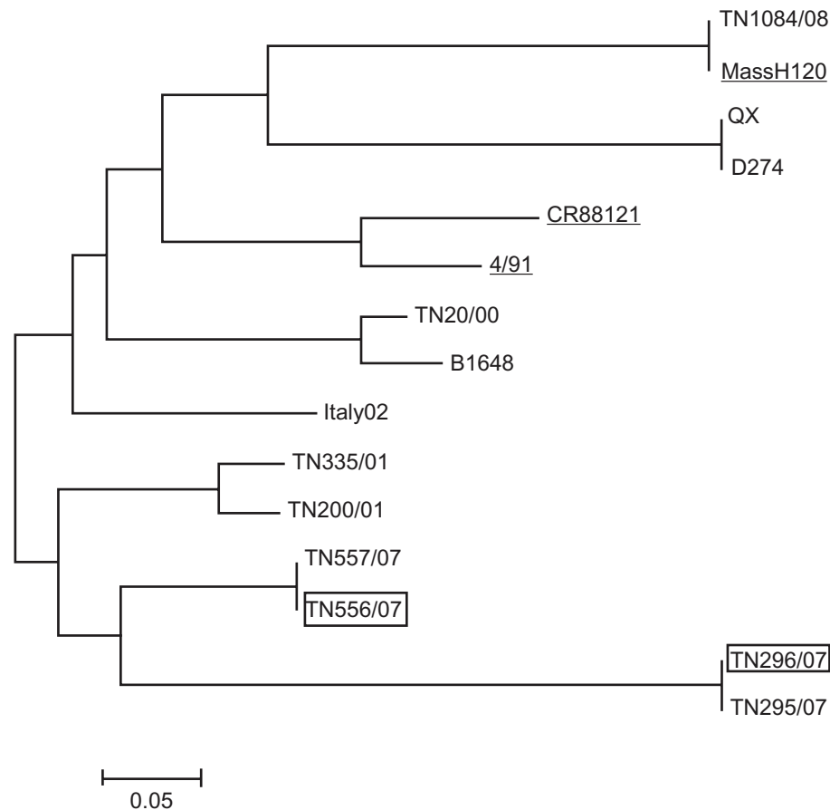
Figure 1 Neighbor-joining phylogenetic tree with 1000 bootstrap replicates expressing the relationships among deduced S1 amino acid sequences of TN296/07 and TN556/07 with selected infectious bronchitis virus reference strains.
