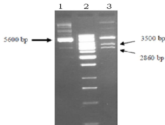
Figure 1. Results of enzymatic digestion of pcDNA3.1Hygro p24-gp41 for confirming the presence of p24-gp41. Lane 1, undigested plasmid, lane 2, 1kb DNA marker, lane 3, plasmid digested with NdeI .
