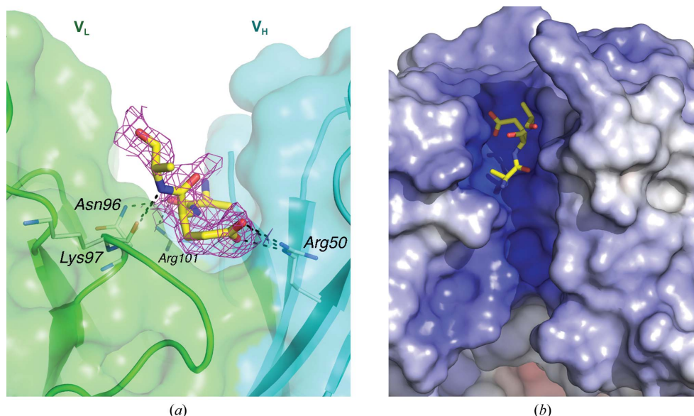
Figure 4 Human IgG1 \kappa Fab in complex with an antigenic peptide. (a) \sigma_A -weighted 2mF_{\text{obs}} - DF_{\text{calc}} electron-density map of FabG contoured at 1\sigma . For clarity, the map is only shown around the visible residues of the antigenic peptide. Some of the polar interactions with paratope residues are depicted as dashed lines. A detailed description is given in the main text. (b) Molecular surface of FabG coloured by electrostatic potential as mapped onto the solvent-accessible surface (colour ramp from -10k_B T/e_c in red to 10k_B T/e_c in blue, where k_B is the Boltzmann constant, T is the absolute temperature and e_c is the charge of one electron). The model shown corresponds to the peptide-complexed protein, although the peptide residues were removed for the Poisson–Boltzmann electrostatic potential calculation.
