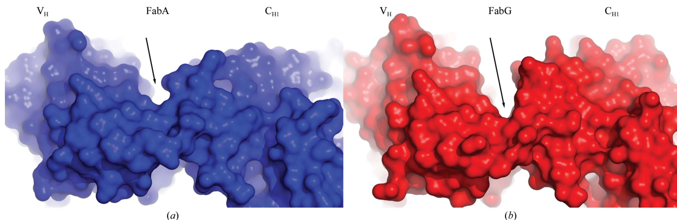
Figure 5 FabA versus FabG V H –C H1 interfaces. The solvent-accessible surfaces of (a) human IgA1 \kappa FabA and (b) IgG1 \kappa FabG are shown in blue and red, respectively. The models are shown in an identical orientation viewed from the heavy-chain side. The arrows highlight the difference in the tightness of interaction between the two domains in the two different Ig isotypes.
