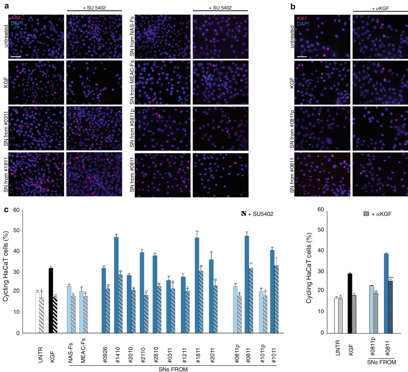
Fig. 4 Reduction of the SN proliferation effects by inhibition of the KGFR activity or block of the KGF binding to the receptor. HaCaT cells were serum-starved, treated with SNs or with KGF for 48 h at 37 °C in presence of the specific FGFR tyrosine kinase inhibitor SU5402 ( a ) or of the neutralizing anti-KGF antibodies ( b ), fixed and immunostained with anti-Ki67 polyclonal antibodies. Quantitative immunofluorescence analysis indicates that inhibition of the KGFR activity as well as block of the KGF binding to the receptor induce a reduction in the percentage of cycling cells in response to the different SNs. The reduction is more evident after treatment with SNs from
