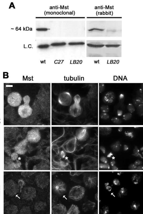
Fig. 8. Mst accumulates in mitotic cells. (A) Western blot of larval brain extracts from wild-type (wt), mst C27 and mst LB20 mutants. Both the monoclonal (Santa Cruz) and the polyclonal (rabbit) antibodies recognize a single band of approximately 64 kDa, which is absent in mutant brains. Giotto (Giansanti et al., 2006) was used as loading control (L.C.). (B) Localization of Mst in wild-type and mst larval brains. During mitotic division, both neuroblasts and GMCs (asterisk) exhibit a strong and diffuse Mst signal, which persists from prophase to telophase; this signal is very weak in interphase cells. Mitotic cells of mst mutants (arrows) do not display any staining, confirming the specificity of the antibody. Scale bar: 5 \mu m.
