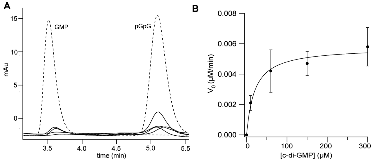
Figure 2. c-di-GMP hydrolytic activity of PA4108. (A) Representative time-courses of pGpG and GMP formation obtained after incubation of 0.64 μM PA4108 with 150 μM c-di-GMP (in the presence of 10 mM MgCl 2 and 2.5 mM MnCl 2 ). The nucleotide content of the reaction mixture was analyzed by RP-HPLC at different times (30, 60, 100, 180 min, at 30°C; solid lines in the figure) and compared with a calibration curve of standard solutions of GMP and pGpG (the chromatogram of a 5 μM solution of both nucleotides is reported as reference, dashed lines). (B) Plot of the initial rate of c-di-GMP hydrolysis (μM of c-di-GMP consumed/min) measured at different c-di-GMP concentrations (black circles). Data were fitted with the Michaelis-Menten equation (continuous line) in order to extrapolate the K_M and V_{max} parameters (20 μM and 5.8 \times 10^{-3} μM/min, respectively). Data are the average of at least two independent experiments.
