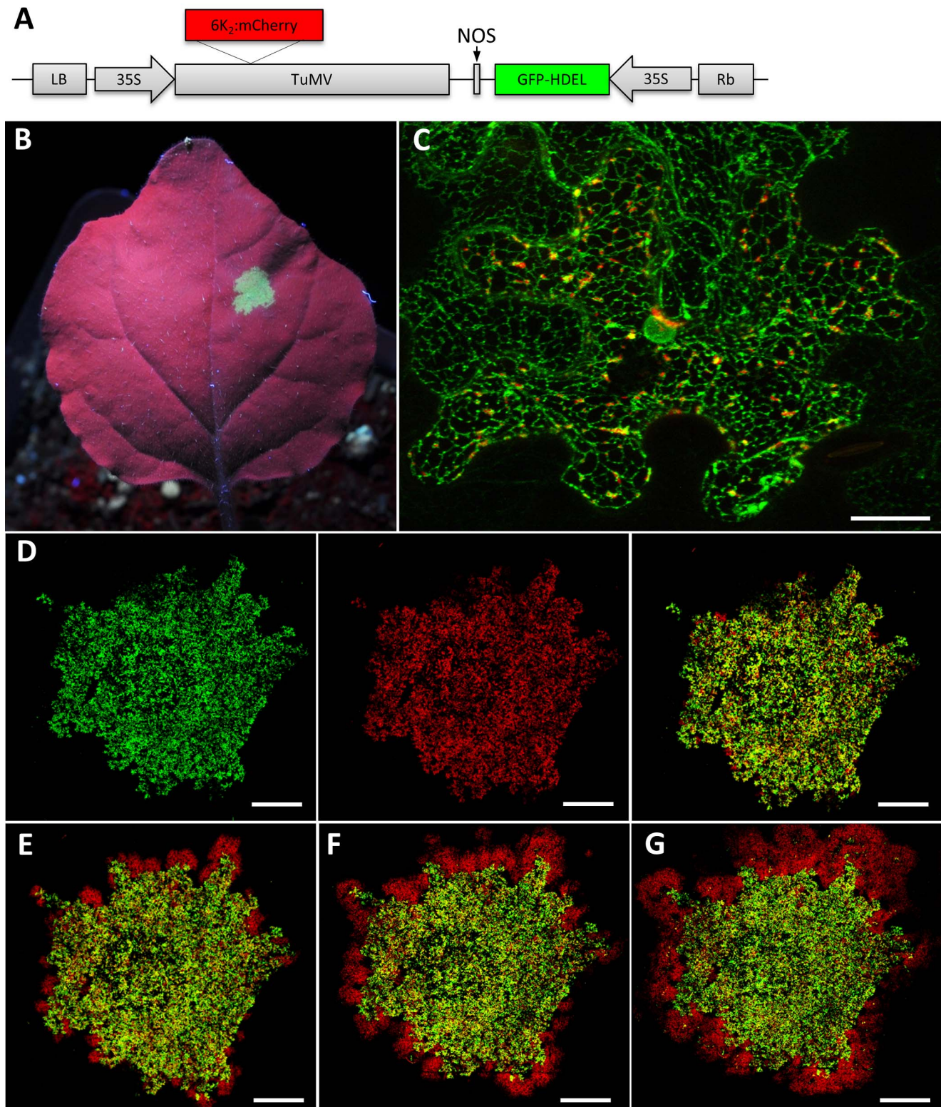
Figure 1. TuMV intercellular movement time course. (A) Schematic representation of the plasmid pCambiaTuMV/6K2:mCherry/GFP-HDEL used to discriminate primary infected cells from secondary infected cells after agroinfiltration. cDNA coding for 6K2:mCherry was inserted between P1 and HCPro cistrons. (B) Image of a leaf under uv illumination. Green fluorescent zone shows agroinfiltrated area. (C) Three-dimensional rendering of 35 1 µm thick confocal image sections that overlap by 0.5 µm showing the distribution of TuMV-induced 6K2:mCherry-tagged structures and GFP-HDEL labeled at 72 hpi. The TuMV-induced 6K2:mCherry-tagged structures represent the viral factories, and the circular green structure in the center of the cell is the nucleus. Scale bar = 20 µm. (D) Three-dimensional tile imaging rendering of N. benthamiana leaf agroinfiltrated 60 hrs before with A. tumefaciens strain Agl1 containing the above plasmid. The confocal image tiles were formed using the 10× objective by assembly 12×12 images in xy and the three-dimensional rendering was created by 5 z stacks of 90 µm thick confocal images that overlap by 45 µm. Left panel, red
