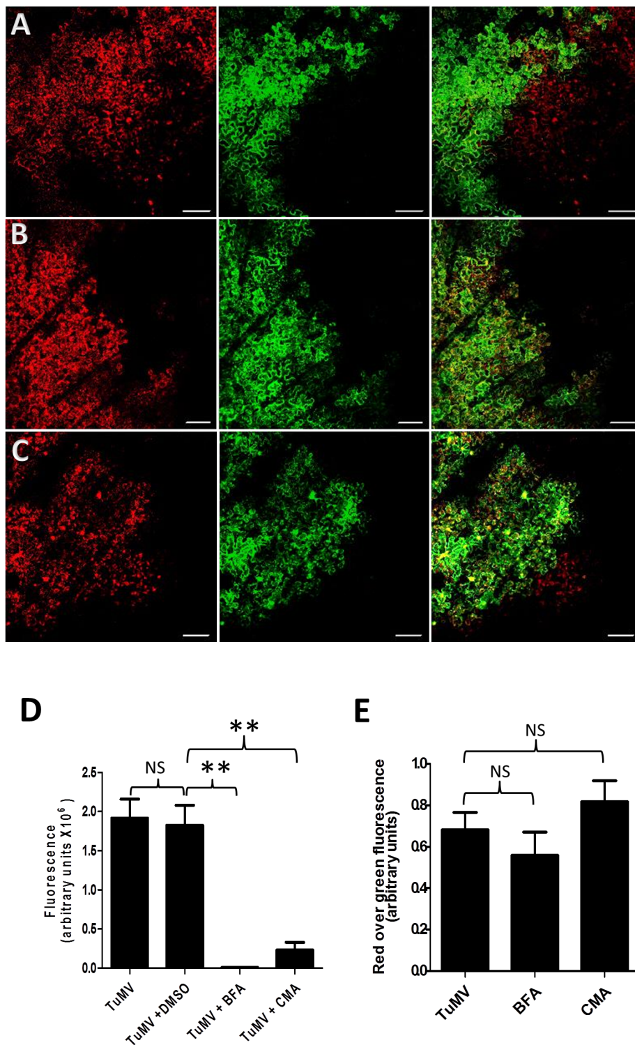
Figure 2. The secretory pathway is required for intercellular movement. N. benthamiana leaves were infiltrated with DMSO (A), 10 \mu g/ml BFA (B) and 0.5 \mu M CMA (C) 4 hours before agroinfiltration with A. tumefaciens containing pCambiaTuMV/6K2:mCherry//GFP-HDEL. All images were taken at 4 dpinf. Left panel, red fluorescence channel imaging TuMV producing 6K2:mCherry; middle panel, green fluorescence channel imaging GFP-HDEL; and right panel, merged images. Scale bar = 200 \mu m. (D) Surface area of red-only fluorescent foci was calculated and expressed in fluorescence units. (E) Fluorescence intensity ratio of red over green foci was calculated and expressed in fluorescence units. Bars represent means and standard errors for 20 replicates per treatment. One-way analysis of variance calculation followed by Tukey's Multiple Comparison Test allowed analysis of differences between means: **, 0.001 < P value < 0.01. doi:10.1371/journal.ppat.1003683.g002
