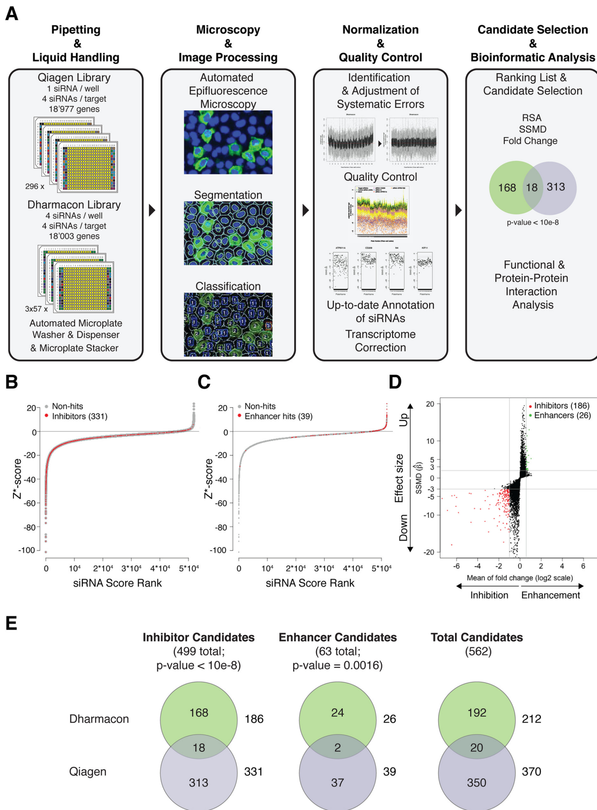
FIG 1 UUKV siRNA screens. (A) Outlines of screening and bioinformatics procedures. (B) Z* score distribution of infection indices obtained for each siRNA in the Qiagen screen regarding inhibitor candidate genes. A redundant siRNA activity (RSA) P value below 0.01 defined potential hits. (C) Z* score distribution, as described for panel B but for enhancer candidate genes. An RSA P value below 0.001 defined potential hits. (D) Dual flash plot for Dharmacon siRNAs, showing selected candidates based on SSMD criteria and the fold change. Inhibitor genes were defined by SSMD and change values below -3 -fold and 0.5 -fold, respectively, and enhancers were defined as those with values above 2 -fold and 1.5 -fold (indicated by the gray horizontal lines). (E) Overlaps of candidate genes between the two siRNA screens. The numbers of potential hits that were specific to the Dharmacon and Qiagen screens are indicated in the top and bottom circles, respectively. The total numbers of potential hits for the Dharmacon and Qiagen screens are indicated next to the top and bottom circles, respectively. The P values, based on Fisher's exact statistical tests, indicate that potential hits obtained for both libraries were not independent.
