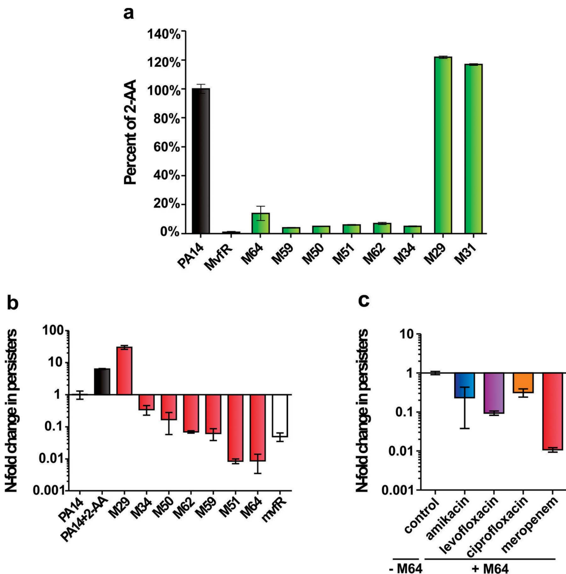
Figure 3. The most potent inhibitors reduce 2-AA production and the formation of antibiotic tolerant persisters. a. 2-AA levels in presence of 10 \mu\text{M} inhibitor. Error bars show mean \pm SD of at least 2 replicates. b. Observed fold change in persister cell concentrations of PA14 cultures with 10 \mu\text{M} inhibitor or with 0.75 mM 2-AA. Untreated PA14 cells and mvfR - cells were the positive and negative controls, respectively. Error bars show mean \pm SEM of at least 3 replicates. Differences between PA14 and the samples M34, M50, M62, M59, M51, M64 or mvfR - ( p < 0.01 ) as well as between PA14 and the samples PA14 + 2-AA or M29 ( p < 0.01 ) are statistically significant (one way ANOVA, Dunnett's test). c. Observed fold change in persister cell concentrations of PA14 plus 5 \mu\text{M} M64 in the presence of clinical antibiotics used to treat P. aeruginosa infections: amikacin (blue), levofloxacin (purple), ciprofloxacin (orange) and meropenem (red). All values were normalized to control cultures in 0.01% DMSO. Error bars show mean \pm SEM of at least 3 replicates. Differences between control and the samples amikacin, levofloxacin, ciprofloxacin or meropenem are statistically significant ( p < 0.01 , one way ANOVA, Dunnett's test). doi:10.1371/journal.ppat.1004321.g003
