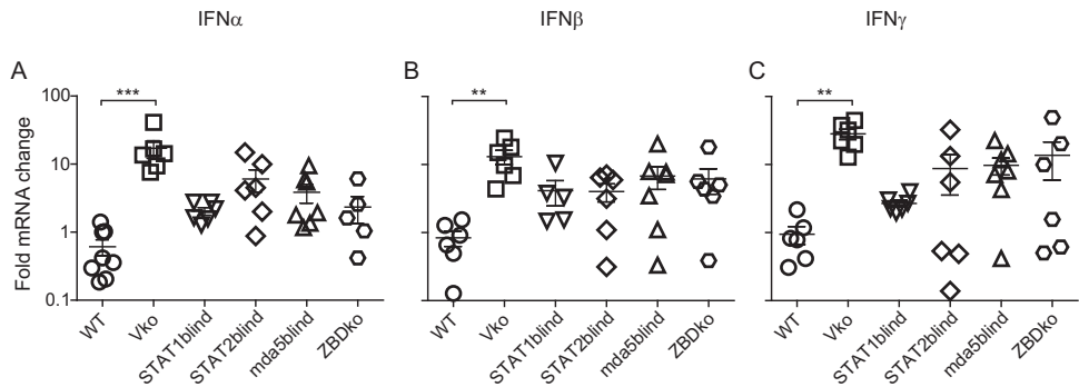
FIG 7 Control of type I and II IFN responses in PBMCs. (A to C) Levels of IFN- \alpha (A), IFN- \beta (B), and IFN- \gamma (C) mRNA expression in PBMCs of animals infected with the parental strain 5804PeH (WT), the Vko derivative, or the different mutant viruses. RNA was isolated from PBMCs on day 0 and 3 postinfection, and PCR assays were conducted using primers specific for the genes indicated at the top of each panel (IFN- \alpha , IFN- \beta , and IFN- \gamma ). The fold change ratios between experimental and control samples for each gene were calculated and normalized against GAPDH using the \Delta\Delta C_T method. Error bars represent the SEM. Asterisks show the levels of statistical significance as follows: **, P < 0.01 ; ***, P < 0.001 .
