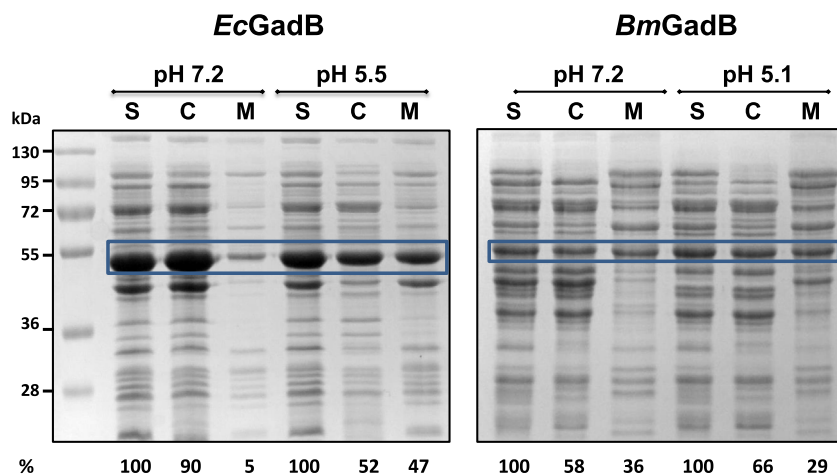
Fig. 7. pH dependent cellular partition in EcGadB (left panel) and BmGadB (right panel). 12% SDS–PAGE of 30 µg-samples of cell supernatants (S), obtained after cell lysis, cytoplasmic (C) and membrane (M) fractions obtained as described in Section 2.4 at neutral (pH 7.2) and mildly acidic pH (pH 5.5 EcGadB or pH 5.1 BmGadB ). The region of the gel encompassing the bands corresponding to EcGadB and BmGadB is shown with a blue box. Molecular weight (kDa) standards are shown on the right of the left panel. The decarboxylase activity is provided as percentage with respect to the corresponding starting activity in S (100%). The reported activity values represent the mean of 2–3 independent experiments, with a standard deviation not exceeding 10% of the stated value.
