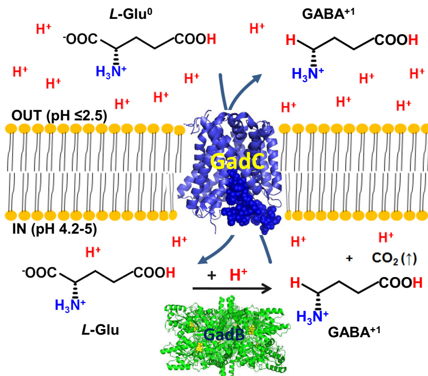
Fig. 1. Schematic representation of the role played by the major structural components of the E. coli GDAR system, the most extensively investigated AR system [1]. \iota -glutamate ( \iota -Glu, net charge 0) is taken up by the electrogenic \iota -Glu 0 /GABA +1 antiporter GadC, an inner membrane protein. Decarboxylation of \iota -Glu via GadA/B consumes an intracellular H + at each catalytic cycle, while GadC contributes to the generation of proton motive force by GABA (net charge +1) export. The structures of GadB at acidic pH (PDB: 1PMM) and GadC at pH 8.0 (PDB: 4DJK), the only one currently available, are shown as ribbon drawing generated with PyMol. The C-plug that in GadC is locking the substrate entry channel is shown in filled space.
