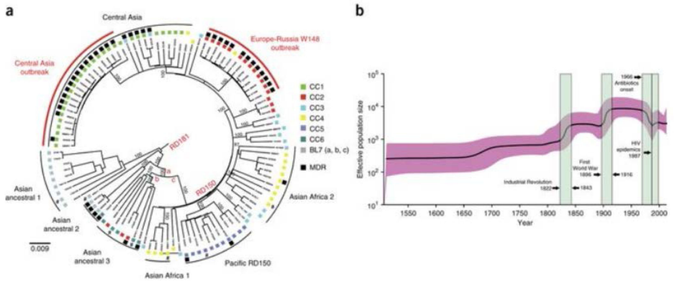
Figure 2: Phylogenetic reconstruction of the MTBC Beijing lineage and change in population size through time.
