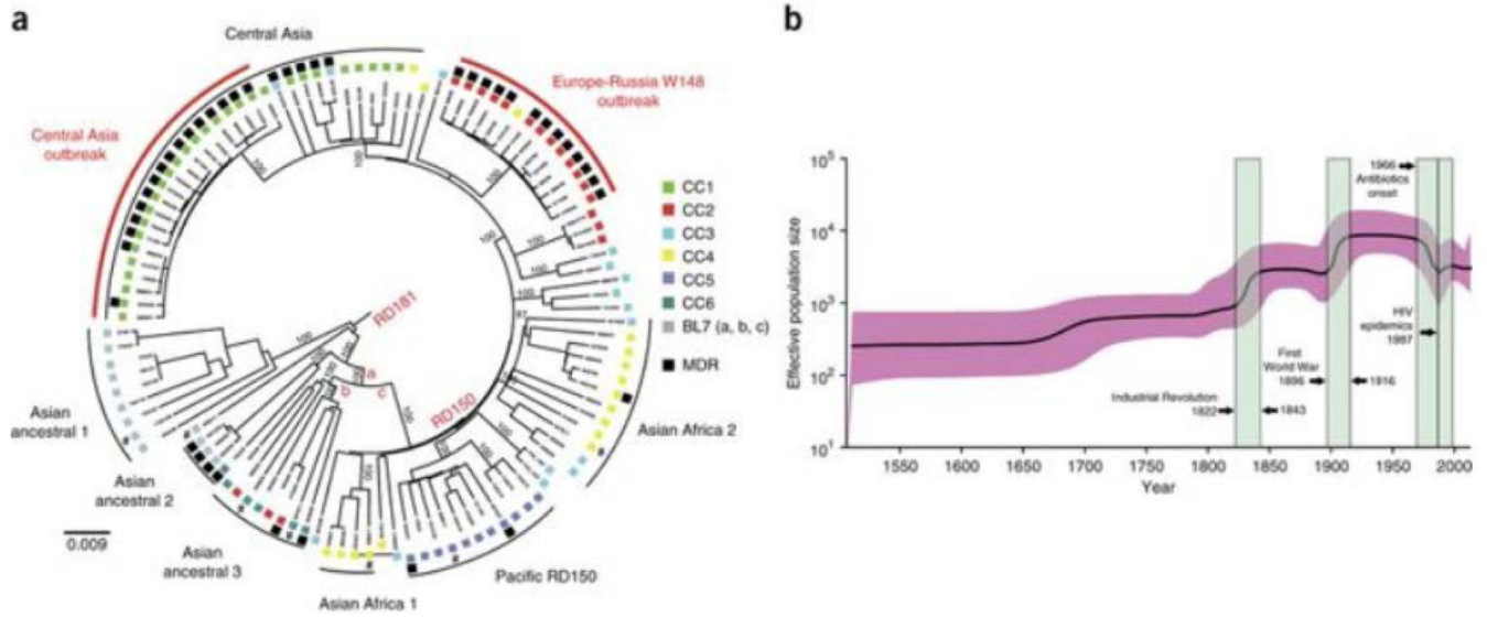
Figure 2: Phylogenetic reconstruction of the MTBC Beijing lineage and change in population size through time. (a) Midpoint-rooted maximum-likelihood tree based on 110 genomes and a total of 6,001 concatenated SNPs. Characteristic mutations differentiating modern and ancestral Beijing strain types are mapped on the tree—mutT4 encoding p.Arg48Gly (branch a), ogt encoding p.Arg37Leu (branch b) and mutT2 encoding p.Gly58Arg (branch c)—as is the absence of the RD181 and RD150 regions of difference. Black squares correspond to strains with an MDR or extremely multidrug-resistant (XDR) phenotype, and a number sign indicates strains lacking drug susceptibility test information. Numbers on branches correspond to bootstrap values. The tree topology remains the same when H37Rv is used as an outgroup. (b) Bayesian skyline plot indicating changes in the Beijing lineage over time with a relaxed molecular clock set at 1 \times 10^{-7} mutations per nucleotide per year. The shaded area represents the 95% confidence intervals, and the green colored boxes represent major socioeconomic events that might have affected the demography of M. tuberculosis .
