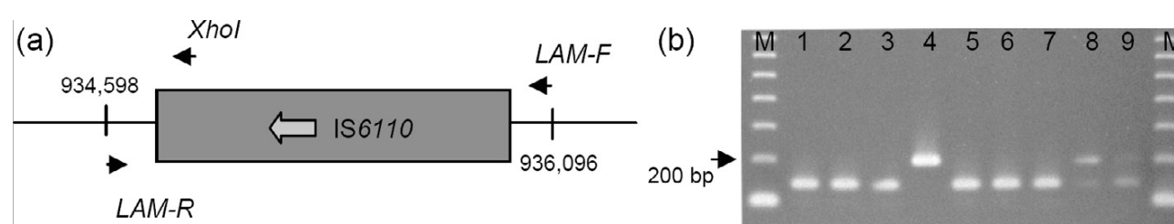
Fig. 3 – LAM-specific PCR: (a) schematic view of the genome region harboring LAM-specific IS6110 insertion in complete genome of strain F11. Three primers (arrows) are used in one reaction: LAM-F, LAM-R, XhoI. Non-LAM strain (without this IS6110-insertion): primers LAM-R and LAM-F amplify 141 bp fragment. LAM strain (with this IS6110 insertion): primers LAM-R and XhoI amplify 205 bp fragment (b) gel-electrophoresis. Lane 4 – LAM strain; lanes 8–9: mixed profile. M, molecular weights marker “100 bp DNA ladder” (GE Healthcare).
