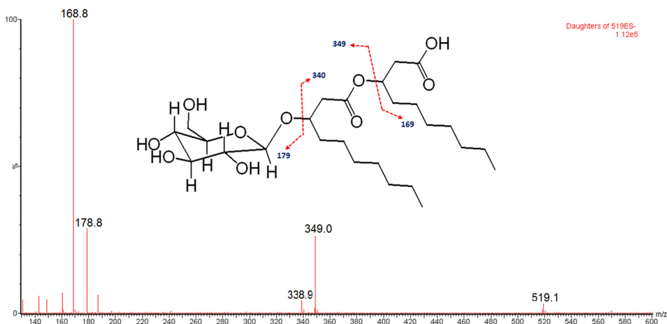
FIG 5 Daughter ions produced upon fragmentation of the m/z 519 pseudomolecular ion, using MS/MS. The proposed structure and fragmentation pattern are illustrated.
