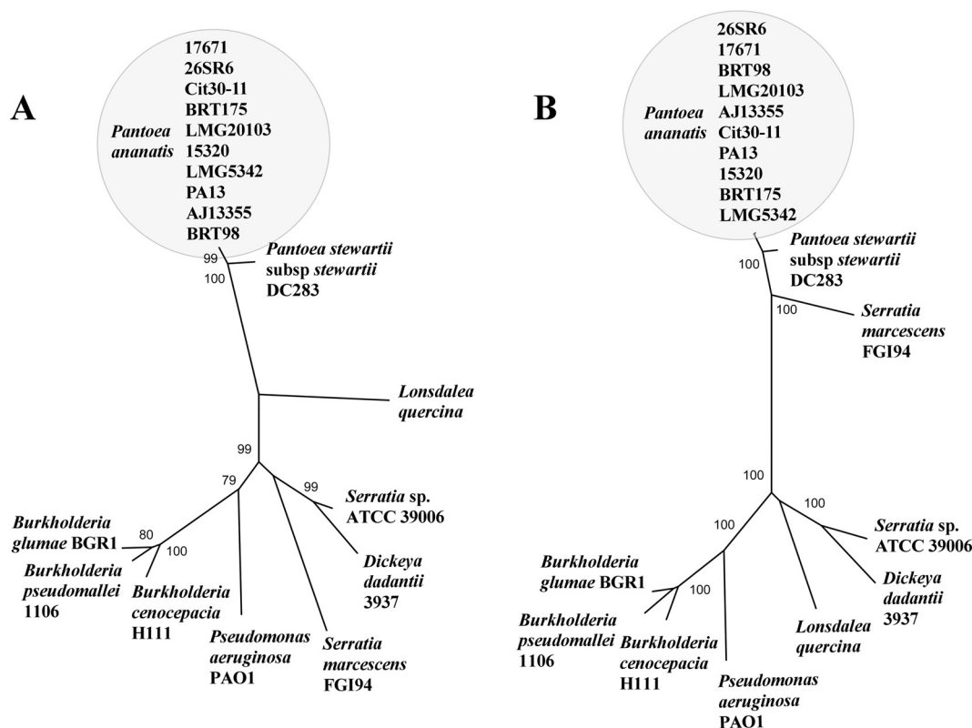
FIG 8 Phylogenetic trees of RhlA and RhlB homologs. Radial (unrooted) neighbor-joining phylogenies of representative RhlA (A) and RhlB (B) homologs, constructed using the Jones-Taylor-Thornton amino acid model, with complete gap deletion. Only bootstrap values greater than 70% are shown. In addition to the P. ananatis strains used in this study, other representative taxa included Burkholderia cenocepacia H111 (CDN64069), Burkholderia glumae BGR1 (ACR31008), Burkholderia pseudomallei 1106a (ABN94800), Dickeya dadantii 3937 (YP_003882762), Lonsdalea quercina (WP_026742016), Pantoea stewartii subsp. stewartii DC283 (EHU02365), Pseudomonas aeruginosa PAO1 (NP_252169), and Serratia marcescens FGI94 (AGB82844).
