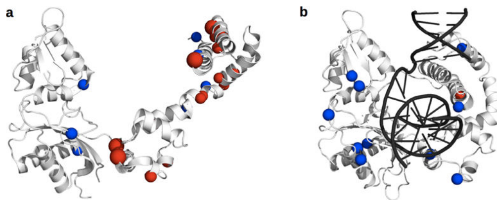
Figure 6. Conformational exchange experienced by Pol β. Residues displaying elevated R_2 and ^{15}\text{N} -CPMG relaxation dispersion curves are shown as blue and red spheres, respectively, corresponding to Cα atoms. (a) The apo form shows millisecond dynamics predominantly in the lyase domain (residues 1–90). Residues with k_{ex} \sim 1400 \text{ s}^{-1} are shown as smaller spheres while residues with k_{ex} \sim 4000 \text{ s}^{-1} are shown as larger red spheres. Few residues in the other polymerase domains show elevated R_2 values; (b) Only residue Glu21 displays ^{15}\text{N} -CPMG relaxation dispersion in the binary form. Other residues displaying elevated R_2 values are located in the polymerase domain of Pol β. DNA in the binary form is shown in black. The relaxation data used for preparing this figure were taken from reference [8].
