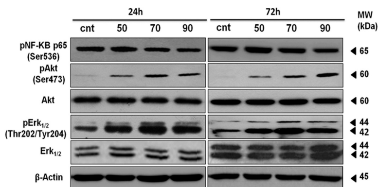
Figure 5. Mertensene induces ERK-1/-2, AKT and NF- \kappa B activation in HT29 cells. Cells were treated with vehicle or with mertensene (50, 70 and 90 \mu\text{g/mL} ) for 24 h and 72 h. Protein extracts (30 \mu\text{g} ) prepared were analyzed by Western blotting using the indicated antibodies. \beta -Actin was used as a loading control.
