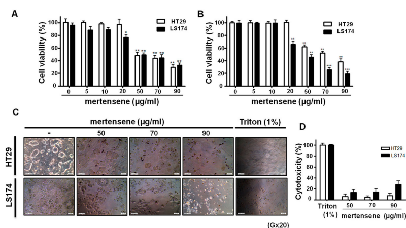
Figure 2. Mertensene inhibits HT29 and LS174 cell viability. Cells were treated with increasing concentrations of mertensene (50, 70, 90 µg/mL) for 72 h. Cell viability was analyzed by MTT assay (A) and trypan blue method (B). The morphological changes were detected by microscopic observation (C) and the cytotoxicity was evaluated by LDH assay (D). Values are means ± S.D. from three independent experiments. Statistical differences were analyzed with Student's t -test (* p < 0.05, ** p < 0.01, *** p < 0.001).
