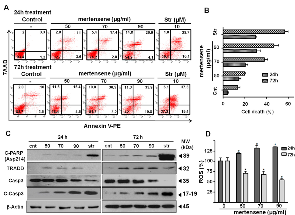
Figure 4. Mertensene induces apoptotic cell death and modulates reactive oxygen species (ROS) accumulation in HT29 cells. Cells were mock- or mertensene-treated at concentrations of 50, 70, 90 \mu\text{g/mL} for 24 h and 72 h. (A) Flow cytometric analysis of apoptotic cells after annexin V/7-AAD staining of mock- and mertensene-treated cells. Staurosporine was used as positive control of apoptosis. Bottom left quadrant represents the live cells that are Annexin V - /7AAD - , early apoptotic cells (Annexin V + /7AAD - ; bottom right quadrant), late apoptotic or necrotic cells (Annexin V + /7AAD + ; upper right quadrant), and dead cells (Annexin V - /7AAD + ; upper left quadrant). (B) Data show a dose-dependent increase in the number of apoptotic cells in HT29 cells after treatment with mertensene. (C) Protein extracts from whole cell lysates were analyzed by Western blot using the indicated antibodies. Anti-actin was used as loading control. (D) ROS production was evaluated by detection of fluorescence using the fluorogenic probe CMH2DCFDA after 24 and 72 h of treatment with increasing concentrations of mertensene. The results were normalized to mock-treated cells (control). Data represent the means \pm SD of three separate experiments. Statistical differences were analyzed with Student's t -test (* p < 0.05).
