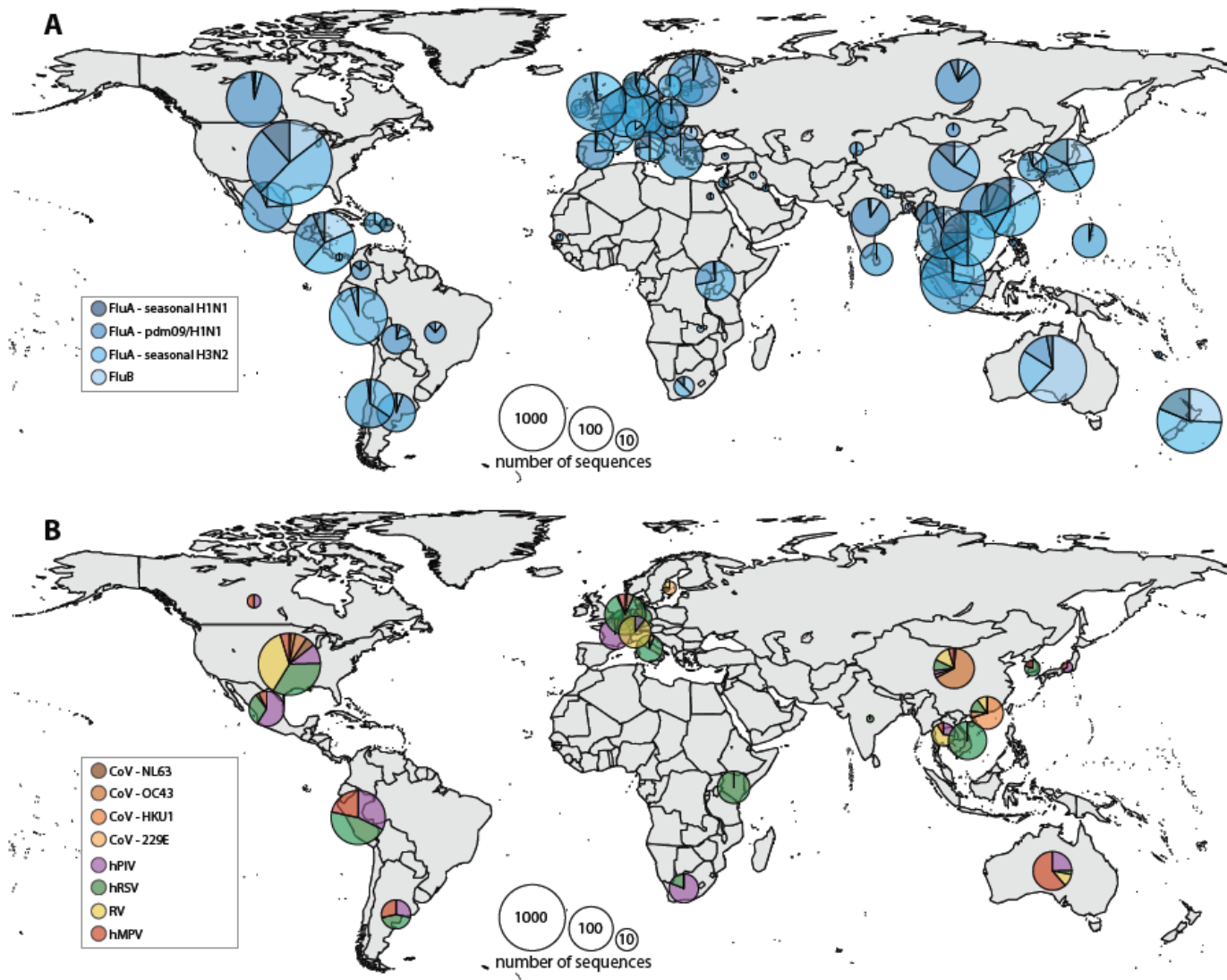
Figure 1. Geographic sources of genome sequence data from different respiratory RNA viruses. Only field strains with complete genome sequences (or nearly complete, >80% of full-length) and geographic information in GenBank ( www.ncbi.nlm.nih.gov/genbank ) were counted (accessed Nov 2015). Panel A shows the counts of human influenza A and B viruses (FluA, FluB). Panel B shows the counts of four human coronavirus (CoV) species (NL63, OC43, HKU1 &
