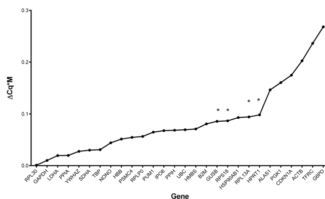
Figure 4. Results from multiplication of the GeNorm M value with the difference of average of Cq results between placental sexes ( \Delta Cq ). A smaller \Delta Cq \cdot M score represents the optimal value for gene expression results normalization for two groups (placental sex). *Genes showing significantly different Cq values between male and female placentas (Student's T test, P \leq 0.05 ; see Fig. 1).
