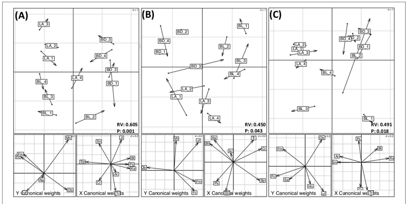
FIGURE 3 | Co-inertia analysis showing the relationship between rhizosphere bacterial and fungal core and eco microbiomes in (A) canola grown as recommended (Can_RE), (B) canola fertilized at 150% of the recommended rate (Can_HF), and (C) canola seeded at 150% of the recommended rate (Can_HD). For each treatment, the top graph is the projection of both bacterial and fungal operational taxonomic units (OTUs) onto the co-inertia plane. The cumulative projective inertias for the first two axes were (A) 92.58%, (B) 96.49%, and (C) 95.88% of the total variation. The label abbreviations are as follows: BL, Beaverlodge; BD, Brandon; LA, Lacombe. Arrow length is proportional to the difference between the ordinations of the two data sets: longer arrows denote less concordance between the two assemblage data sets. The two lower panels are the projection of fungi (left panel) and bacteria (right panel) onto the co-inertia plane for each treatment. The abbreviations for bacterial and fungal species are as follows: Ar, Arthrobacter sp.; Bl, Blastococcus sp.; Cr, Cryococcus sp.; JI, Janthinobacterium lividum ; Ka, Kaistobacter sp.; Ps, Pseudomonas sp.; Sn, Stenotrophomonas sp.; Sp, Serratia proteamaculans ; Tr, Terracoccus sp.; Fc, Fusicolla sp.; Fm, Fusarium merismoides ; Hn, Humicola nigrescens ; Ob, Olpidium brassicae ; Mn, Monographella cucumerina ; Mt, Mortierella sp.; Na, Nectria ramulariae ; uf, unclassified fungus. The RV coefficients are the values of the multivariate generalization of the squared Pearson correlation coefficient. P indicates the P -values of each analysis.
