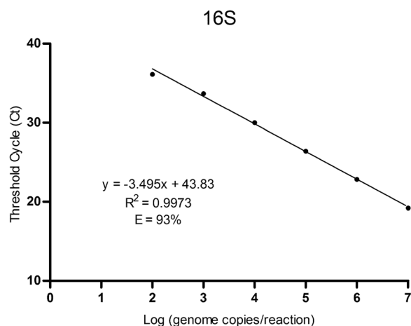
Fig. 3 Standard curve of developed TaqMan-MGB real-time PCR for C. fetus detection. Each point represents the mean Ct of nine different measures (three independent reactions, three replicates each). The curve equation (y), coefficient of determination ( R^2 ) and amplification efficiency (E) are indicated
