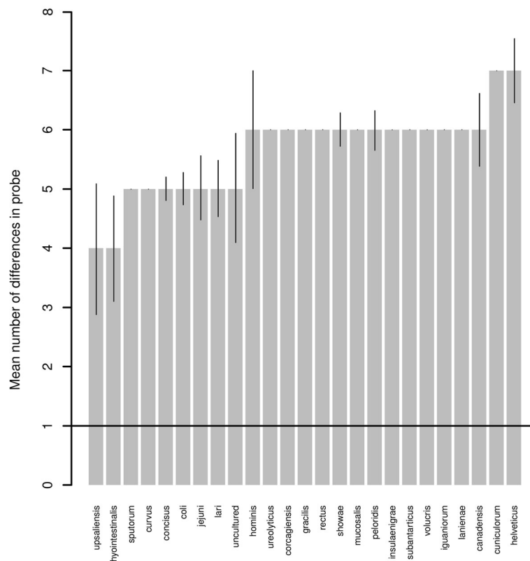
Fig. 2 Mean number of differences in probe sequence of non- C. fetus species 16S gene
