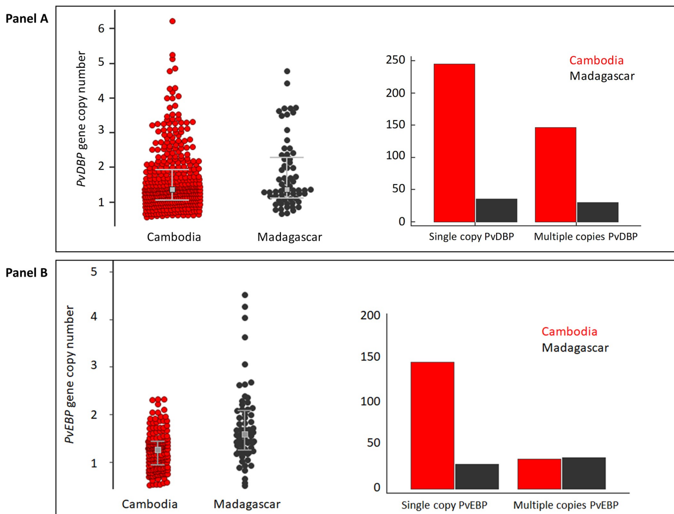
Fig 1. Distribution of PvDBP and PvEBP gene copy number in isolates from Cambodia and Madagascar (Panel A and B, left side). Number of isolates from Cambodia and Madagascar with single or multiple copies PvDBP and PvEBP genes (Panel A and B, right side). The grey squares represent the medians and whiskers the IQRs.
