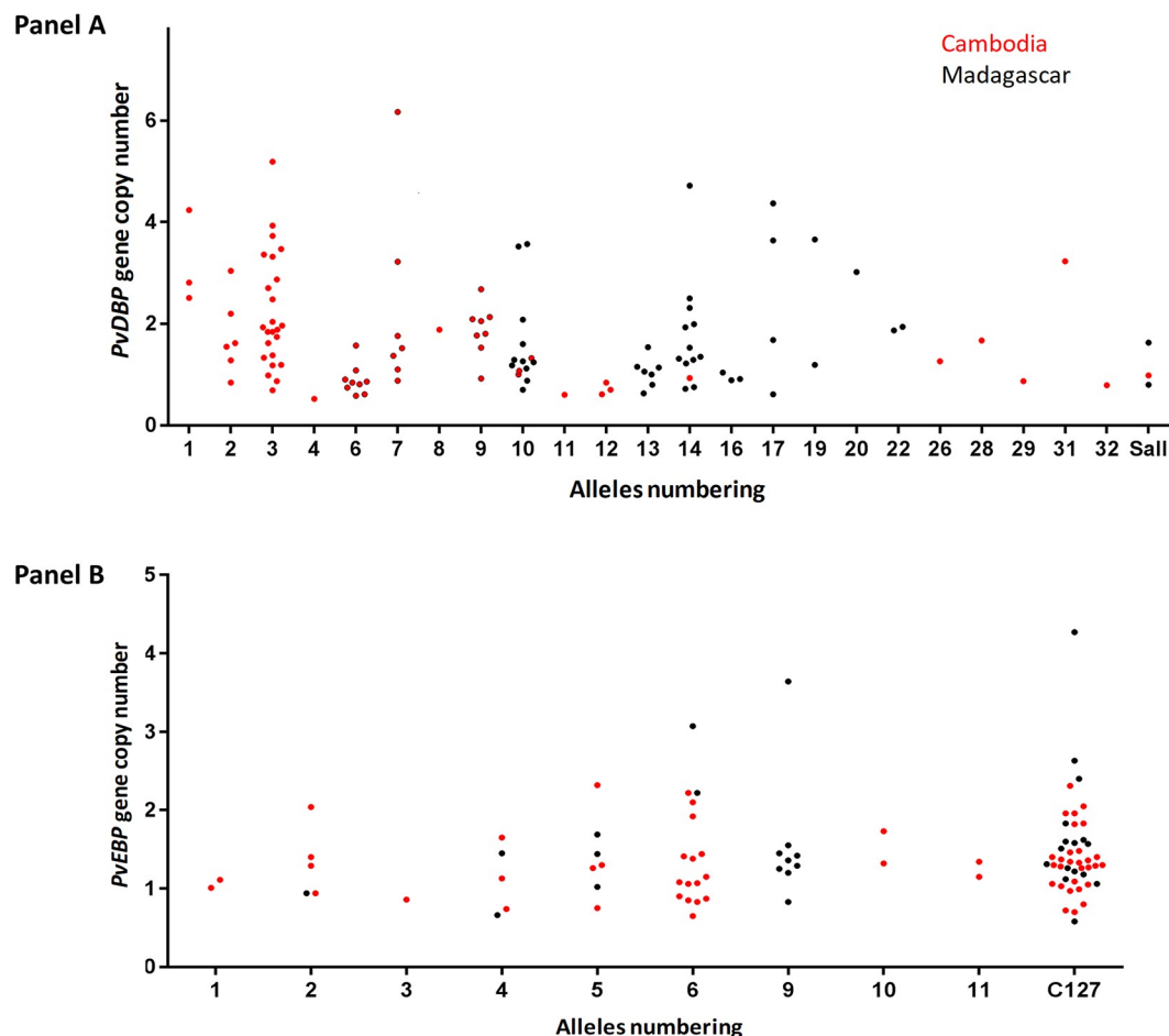
Fig 4. Distribution of PvDBP gene copy number of 33 PvDBP alleles in isolates from Cambodia and Madagascar (Panel A). Distribution of PvEBP gene copy number of 12 PvEBP alleles in isolates from Cambodia and Madagascar (Panel B).
