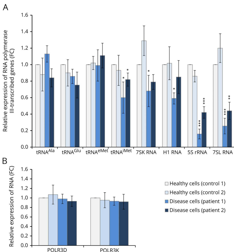
Figure 3 RNA levels determined by RT-qPCR analysis
