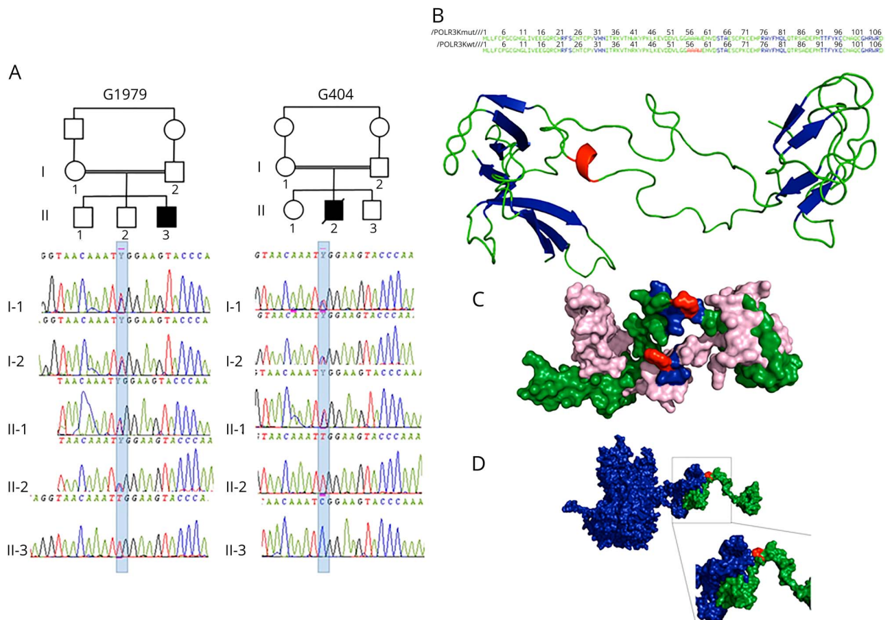
Figure 1 POLR3K mutated families, structural model of POLR3K and of POLR3K-POLR3B interactions
