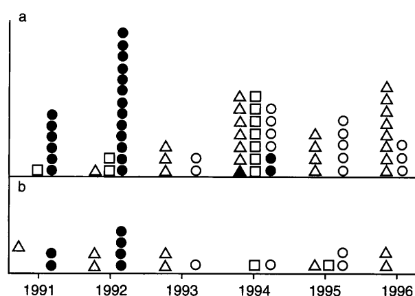
Fig. 1. Serotypes and intratypic differentiation of polioviruses isolated from (a) healthy children and (b) cases of paralytic poliomyelitis: \Delta , vaccine-related type 1; \blacktriangle , wild-type 1; \square , vaccine-related type 2; \blacksquare , wild-type 2; \circ , vaccine-related type 3; \bullet , wild-type 3.
