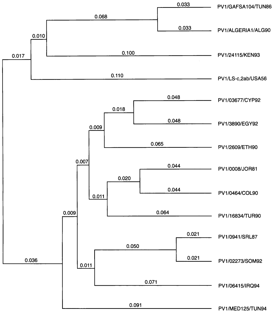
Fig. 3. Sequence relatedness among polio 1 strains. Dendrogram summarising sequence relatedness among polio 1 strains across the nucleotides 3296–3445 in the VP1/2A region [20]. Strain designation and abbreviations are as defined in the legend to Fig. 2.
