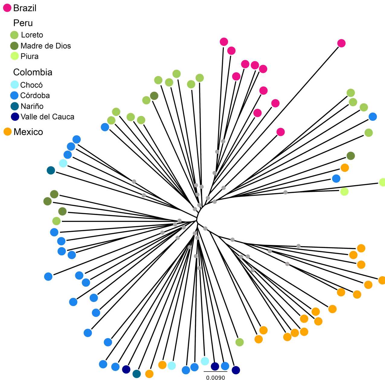
Fig 5. A neighbor-joining phylogenetic tree with 1,000 bootstrap pseudoreplicates obtained with genomic sequences of P. vivax isolates from Brazil (n = 11 isolates), Peru (n = 23), Colombia (n = 31), and Mexico (n = 19). Branch tips were colored according to the geographic origin of samples, as shown in Fig 1. Grey circles indicate internal nodes with > 70% bootstrap support.
