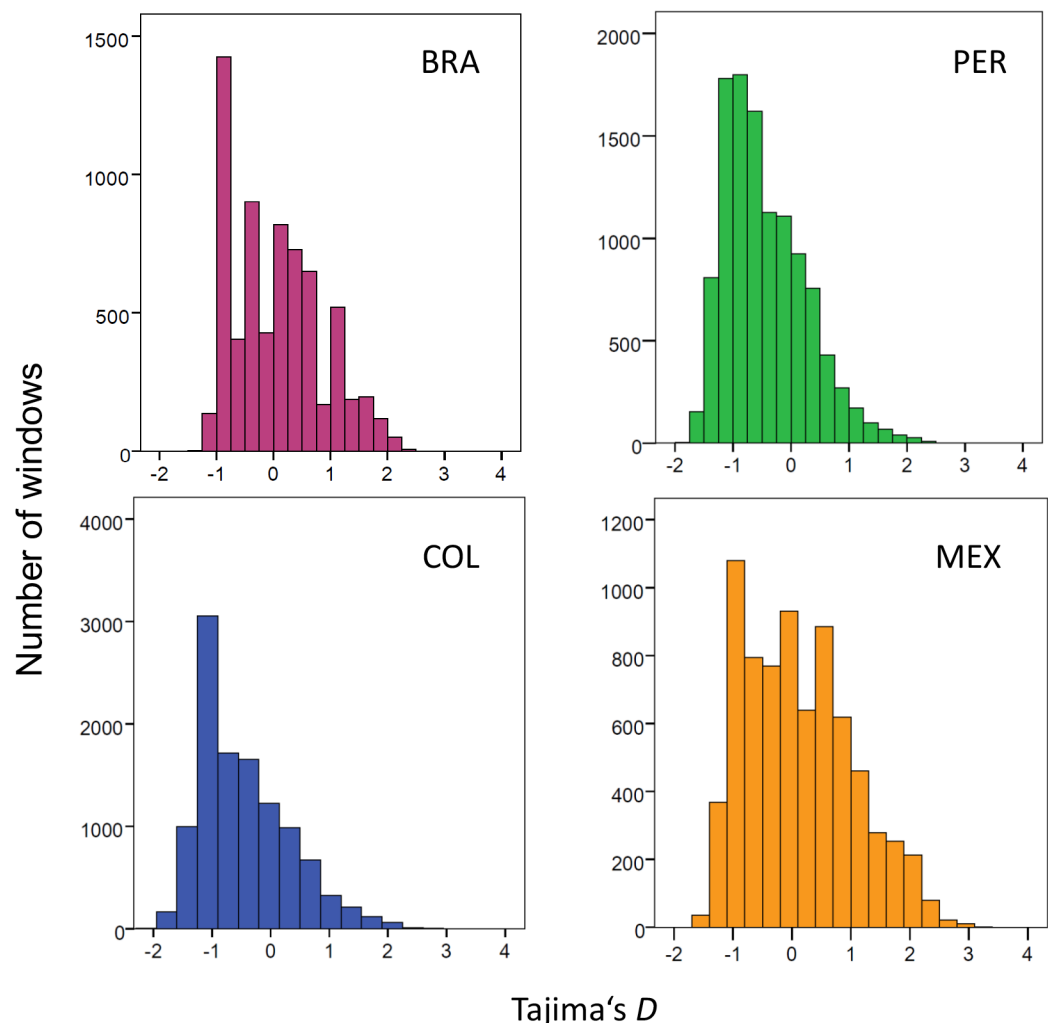
Fig 3. Frequency distribution of Tajima's D values calculated within 1-kb windows of genomic sequence in four New World populations of P. vivax . BRA = Brazil ( n = 11 isolates), PER = Peru ( n = 23 ), COL = Colombia ( n = 31 ), and MEX = Mexico ( n = 19 ).
