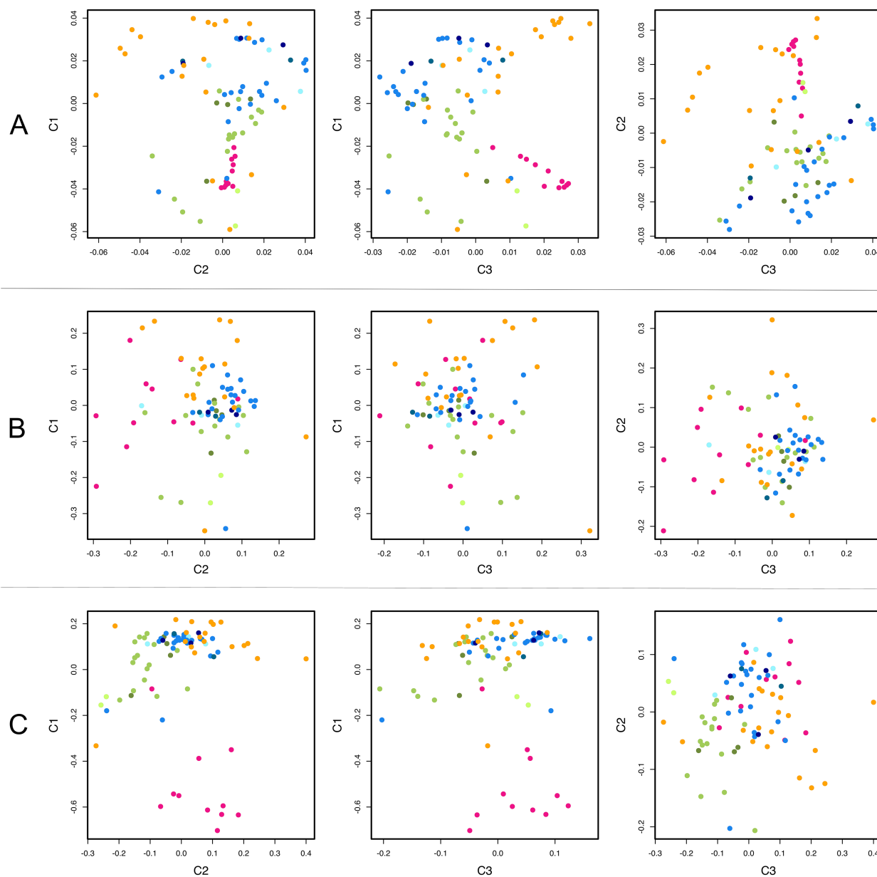
Fig 4. Principal component analysis of the population structure of P. vivax in the New World. Panel A shows results using the complete data set of 94,122 SNPs; panel B shows results obtained with a set of 37 segregating SNPs included in a previously described P. vivax barcode [49]; and panel C shows results obtained with a hypothetical barcode comprising the 100 SNPs yielding the highest average Wright's fixation index F_{ST} values in pairwise comparisons of New World P. vivax populations. The SNPs used in the analysis shown in panel C are listed in S5 Table. Samples are colored according to their geographic origin as shown in Fig 1. The percentage contributions of each principal component (C1, C2, and C3) to overall variance were as follows: panel A, C1 = 22.27%, C2 = 14.15%, and C3 = 8.15%; panel B, C1 = 19.93%, C2 = 12.03%, and C3 = 11.42%; and panel C, C1 = 21.36%, C2 = 10.93%, and C3 = 9.33%.
