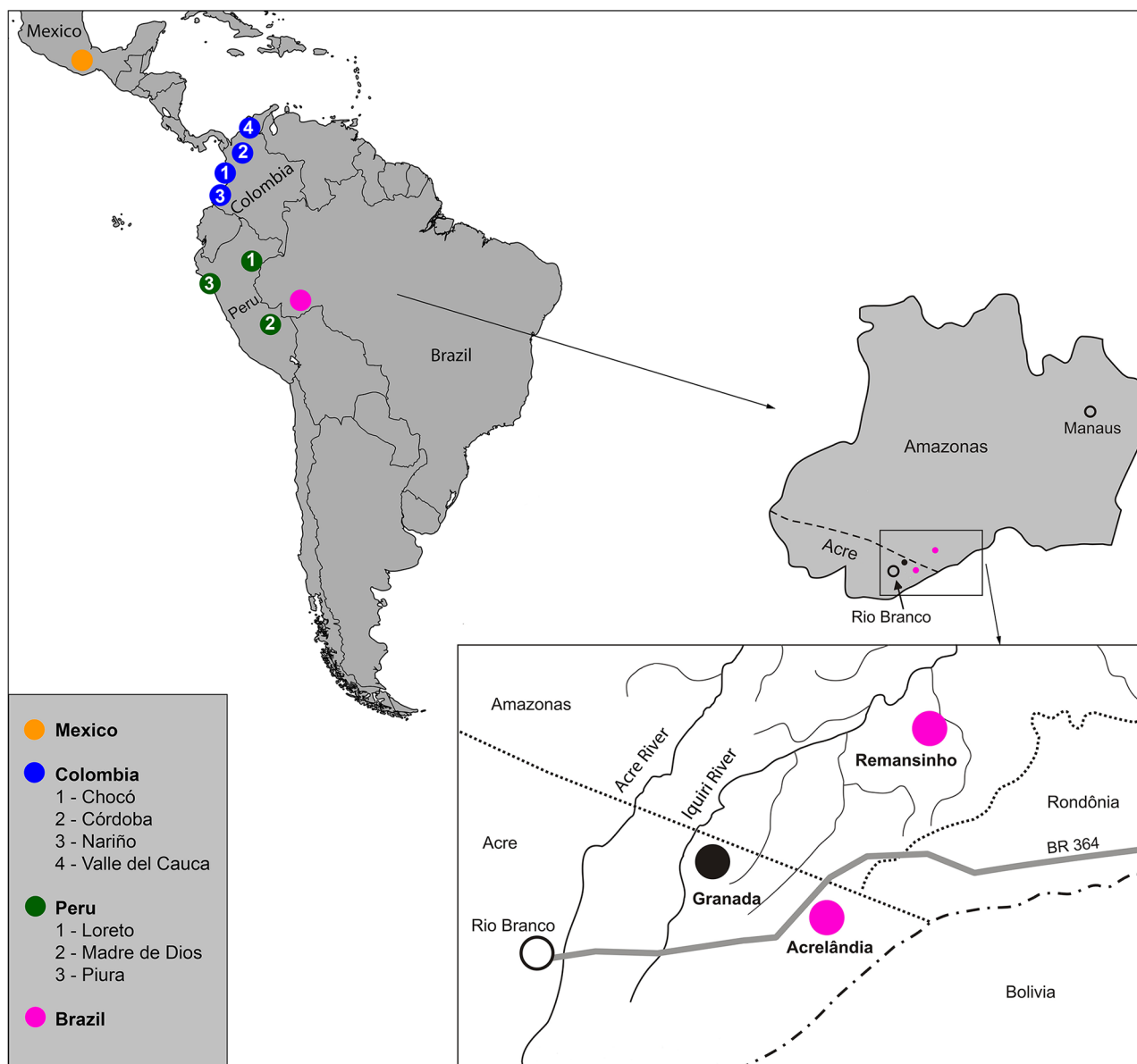
Fig 1. Map showing the sampling locations of the New World P. vivax isolates analyzed in this study, comprising Brazil, Peru, Colombia, and Mexico. The insert shows the study sites in northwestern Brazil (Acrelândia and Remansinho, 120 km apart), close to the border with Bolivia and Peru. Adapted from [15] and https://commons.wikimedia.org/wiki/Atlas_of_the_world#/media/File:BlankMap-World6.svg .
