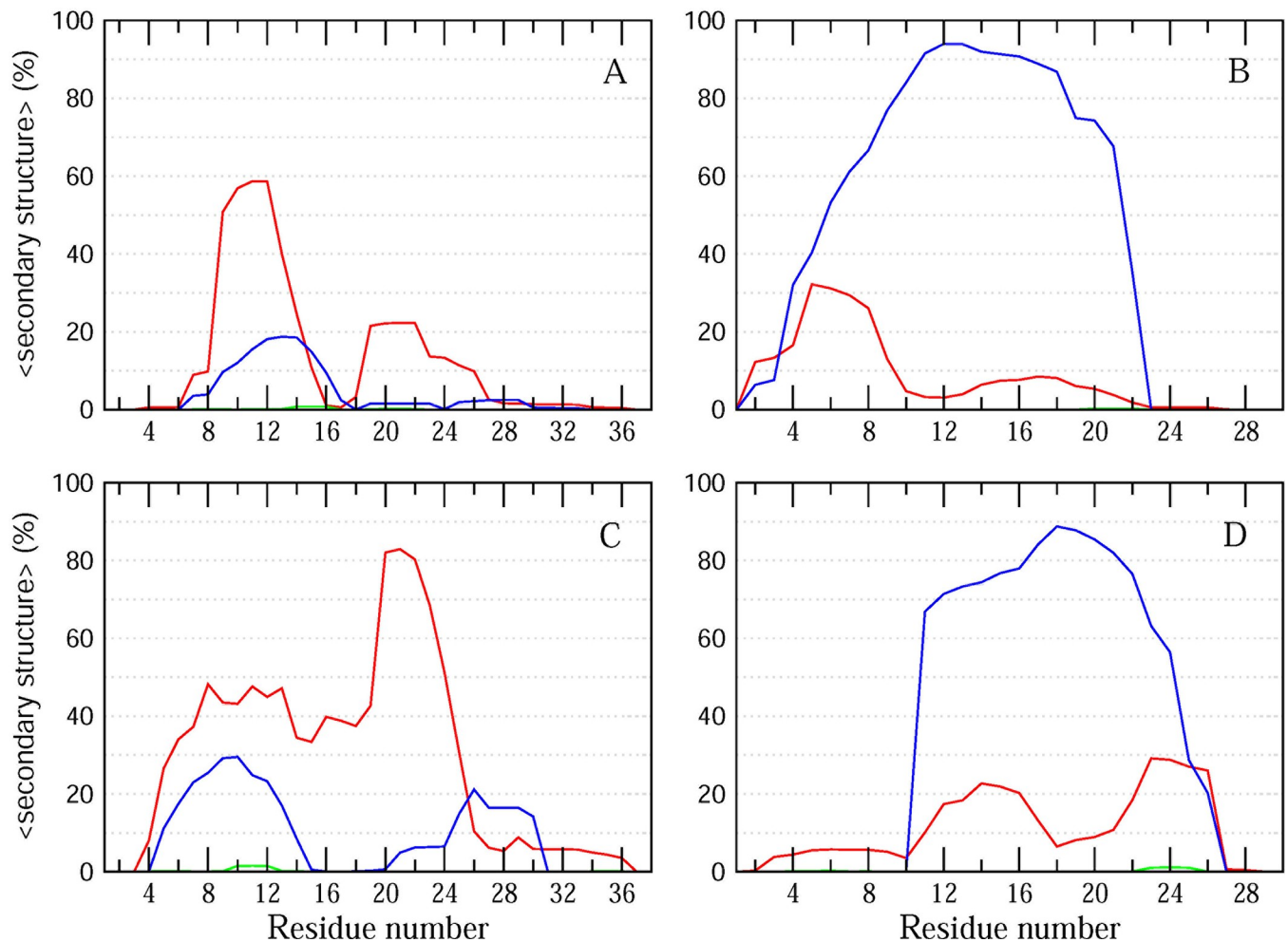
Fig 3. Secondary structural propensities of PACAP38 and PACAP(9–38). The average percent \alpha -helix, 3_{10} and \pi helix as a function of residue number along the sequence are represented as red, green and blue lines, respectively, for two independent MD runs of PACAP38 (A, C) and PACAP9-38 (B, D).
