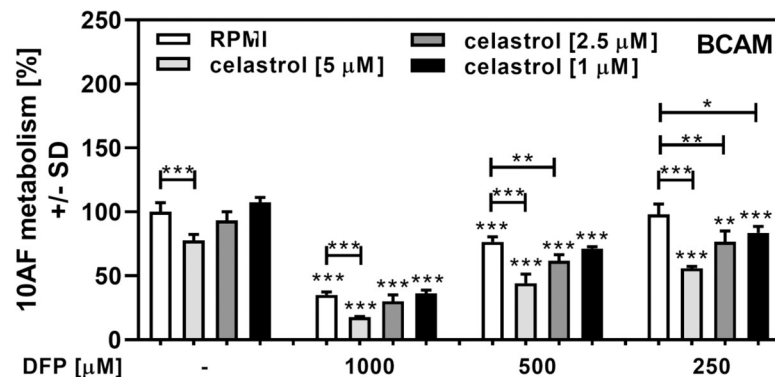
Fig 6. Celastrol sensitizes A. fumigatus for anti-fungal activity of DFP. Forming wildtype A. fumigatus biofilm (10AF) was incubated with 1, 2.5, or 5 \mu\text{M} celastrol, 0.25–1 mM of DFP, or combinations of these two substances at 37°C for 24 hour. Fungal metabolism was measured by XTT assay. Statistics: t-Test. Bars without DFP (leftmost group) vs. all other bars with the same celastrol concentration. Other comparisons as indicated by the ends of the brackets. One, two or three asterisks = p \leq 0.05 , p \leq 0.01 or p \leq 0.001 , respectively.
