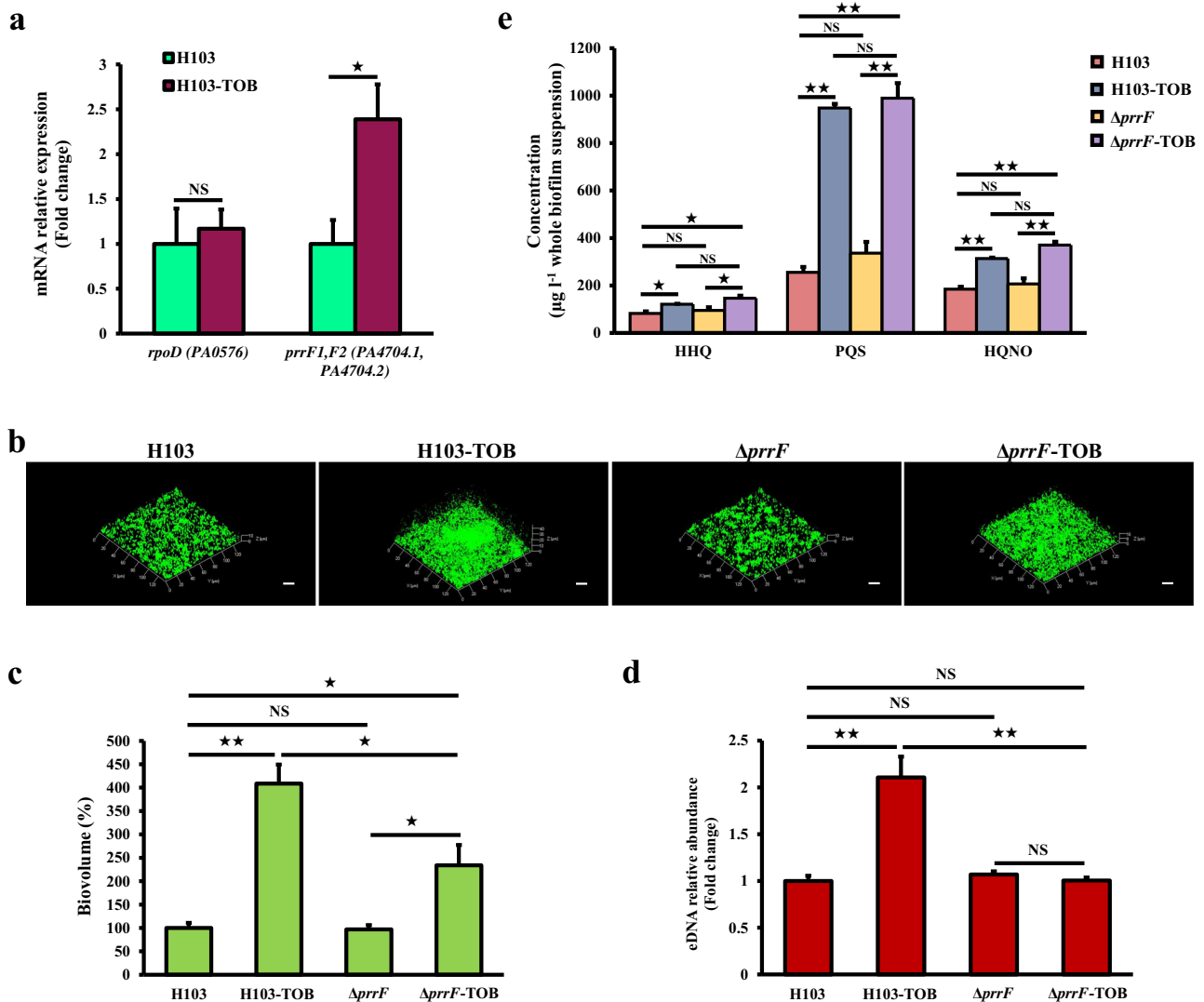
Fig. 5 Role of PrrF1/F2 sRNAs in tobramycin-enhanced biofilm formation. a Relative prfF mRNA levels in P. aeruginosa biofilms exposed to tobramycin (brown bars) compared to the relative expression of mRNA levels in the control condition (green bars), after 24 h of growth. Quantifications have been obtained from at least three independent experiments and rpoD was used as a control housekeeping gene. Error bars represent standard error of the means ( n = 3 ). b Representative CLSM 3D micrographs of 24-h-old biofilms P. aeruginosa H103 and \Delta prfF mutant strains exposed to tobramycin ( 0.8 \mu\text{g ml}^{-1} ) compared to untreated biofilms. Scale bars = 20 \mu\text{m} . CLSM images were analyzed using COMSTAT software to quantify c biofilm biovolumes. Error bars represent standard error of the means ( n = 3 ) and d eDNA relative abundances. eDNA values are normalized to biofilm biomass. Error bars represent standard error of the means ( n = 3 ). e HAQs levels of the \Delta prfF mutant and its isogenic parent strain H103 grown with or without tobramycin supplementation, as determined by LC-MS/MS. Error bars represent standard error of the means ( n = 3 ). Statistics were achieved by a two-tailed t test: ** , P = 0.001 to 0.01 ; * , P = 0.01 to 0.05 ; NS (not significant), P \geq 0.05
