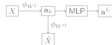
Fig. 4. Classification network &amp; autoencoder.
