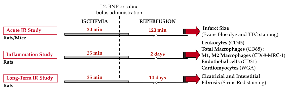
Figure 9. Experimental design. Three protocols of myocardial ischemia-reperfusion (IR) were applied. For acute infarct size study (upper panel), rats and mice underwent 30 min ischemia (full solid line) followed by 120 min coronary reperfusion (thin solid line). In two other additional series of experiments, rats underwent 35 min of ischemia followed by either 2 days (middle panel) or 14 days (lower panel) of reperfusion, to study respectively post-ischemic inflammation and fibrosis. Rats and mice received either B-type natriuretic peptide (BNP, 50 ng/g and 20 ng/g respectively), Lebetin 2 (L2, 100 ng/g and 25 ng/g respectively) or saline (NaCl 9‰, controls), as a single systemic bolus (1 µL/g body weight), 5 min before starting reperfusion.
