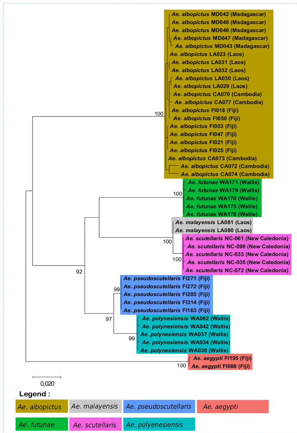
Fig 3. Maximum likelihood evolutionary (MLE) relationships of mosquito species of the Scutellaris Group. Tree derived from 45 concatenated sequences. For analysis, the percentage of replicate trees in which the associated taxa clustered together in the bootstrap test (1000 replicates) is shown for values over 80. The country of collection is indicated along with the specimen number. Colors indicate mosquito species.
