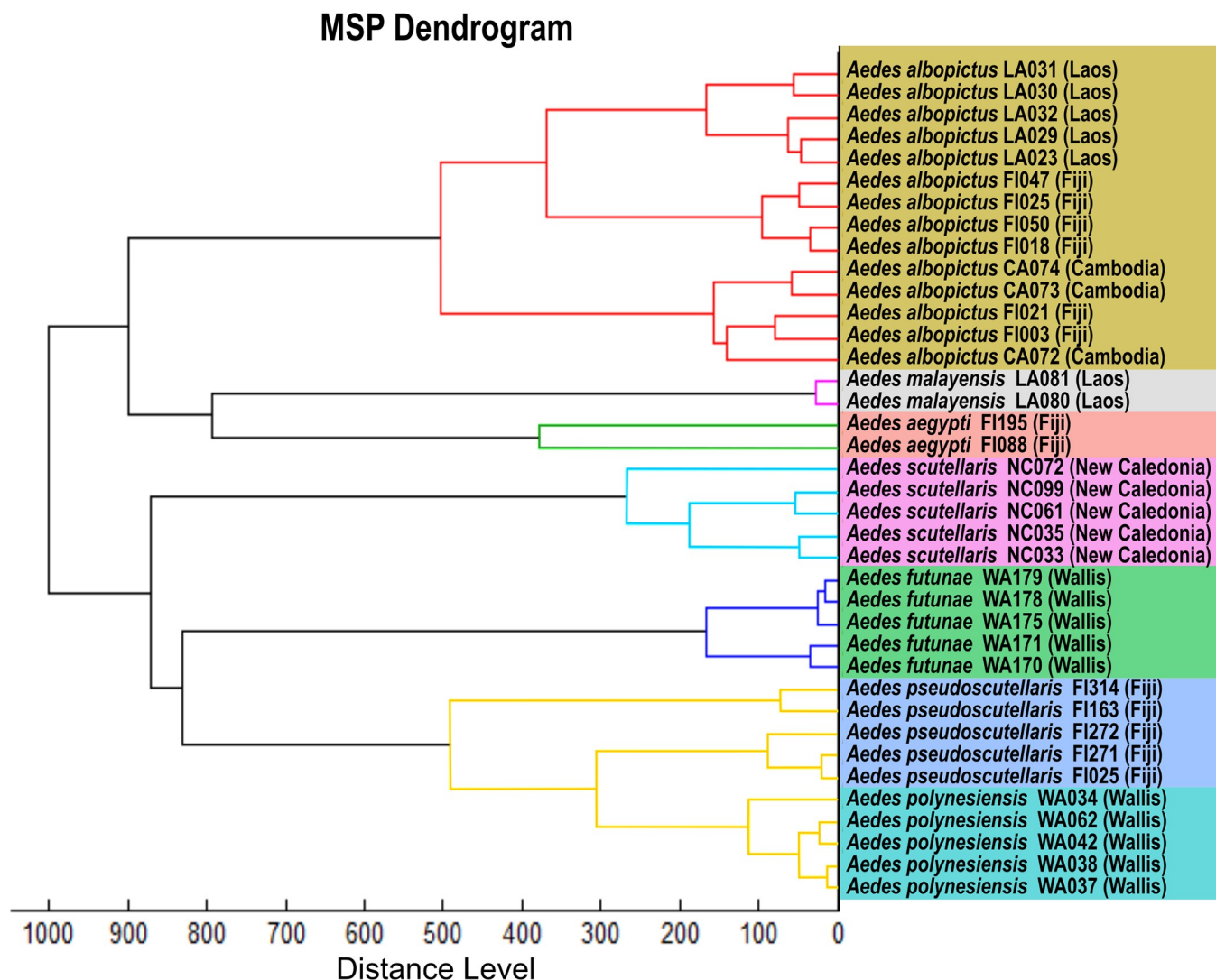
Fig 5. MSP dendrogram of all the mosquitoes belonging to the Scutellaris Group in the MALDI-TOF database. The two Aedes aegypti was used as outgroup taxa. Colors of the branches indicate mosquito species according to the cut-off of 500 (arbitrary units) previously described [41].
