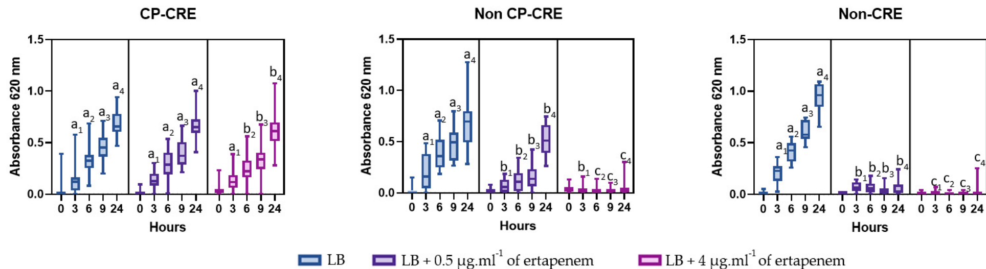
Figure 1. Growth over time according to ertapenem concentration (0, 0.5 or 4 µg.mL -1 ) for carbapenemase-producing-carbapenem-resistant-Enterobacteriales (CP-CRE; n = 57 ), non-carbapenemase-producing-carbapenem-resistant-Enterobacteriales (non-CP-CRE; n = 23 ) and non-carbapenem-resistant Enterobacteriales (Non-CRE; n = 11 ). The same underscored number to a letter reflects time-point specific analyses. Whiskers correspond to min and max values. Different letters above bars indicate significant differences between ertapenem concentration as determined by Fisher's LSD test ( p < 0.05 ).
