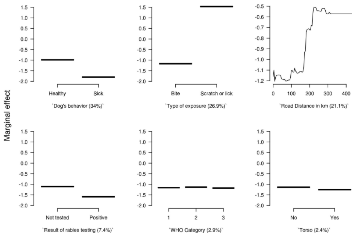
Figure 3: Boosted regression tree and partial dependences graphs showing influence >1% in probabilities after adjustment for other factors and 150-km distance from Phnom-Penh's Doun Penh District, the distance threshold for noncompletion of intended four-session post-exposure prophylaxis protocols, Rabies Prevention Center at Institut Pasteur du Cambodge (rpc@ipc) database 2009-2013. Phnom Penh. Cambodia.
