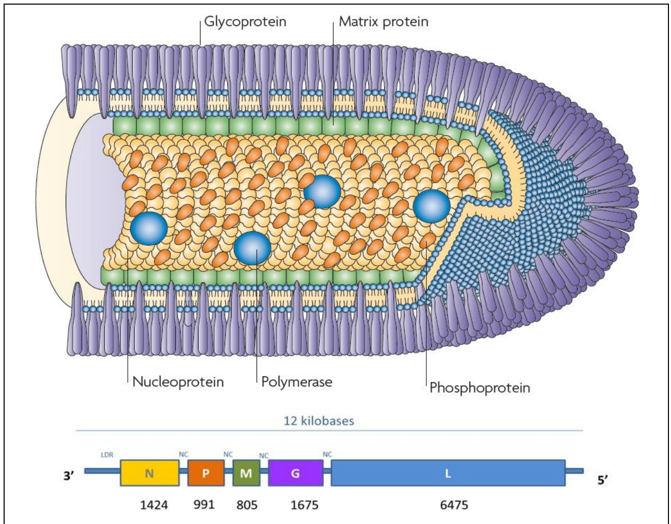
Figure 7: Architecture and functional organization of the rabies virus (adapted from 23,25,494,495 )
